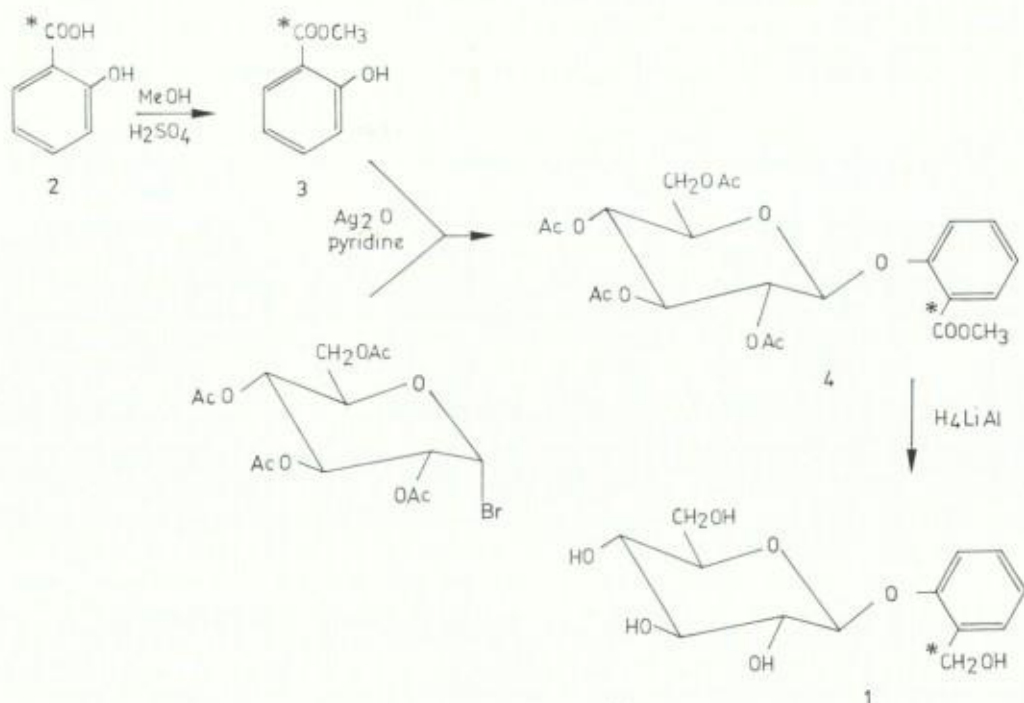
FIG. 1. Scheme of synthesis of [7- 14 C]salicin.
