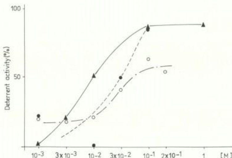
FIG. 2. Deterrent activity of salicin (○, ---), saligenin (●, ----) and salicylaldehyde (▲, —). Calculation of the deterrence index is explained in Material and Methods, section 5.
