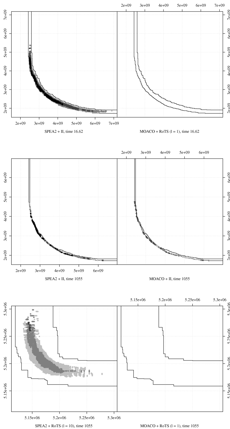
Figure 7. Location of differences in terms of EAFs between SPEA2 and MO-ACO for 16.62 seconds (top) and 1055 seconds (middle) on a structured instance with \xi = 0.0 and for 1055 seconds on an unstructured instance with \xi = 0.75 . The name at the bottom of each plot indicates for which of the two algorithms the differences shown are positive.
