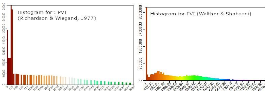
Figure 4. Histograms of pixels' frequency. Left: PVI (Richardson & Wiegand, 1977), right: PVI (Walther & Shabaani, 1991). Plotting: SAGA GIS. Source: author.
