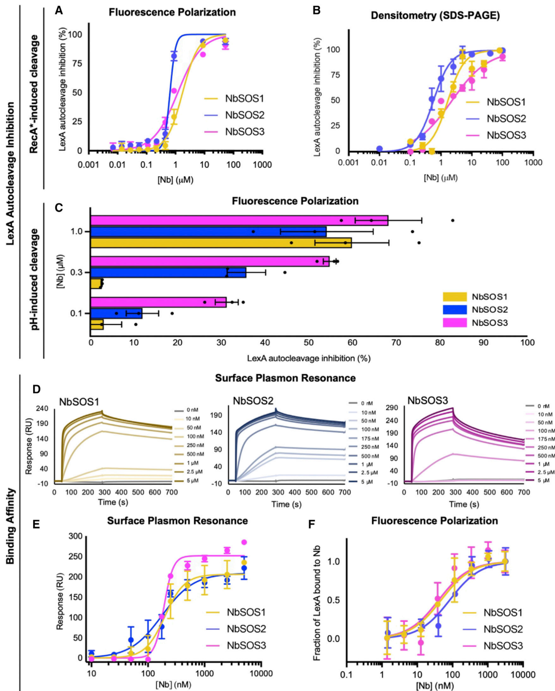
Figure 2. Biophysical characterization of NbSOS1, NbSOS2, and NbSOS3
