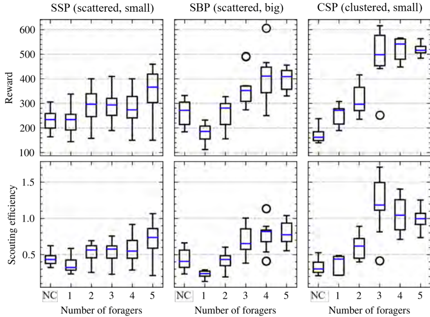
Fig. 4: Performance results for three distributions: SSP (left), SBP (middle) and CSP (right). The top row shows the total reward collected by the swarm at the end of the experiment, and the bottom row the scouting efficiency. The x-axis (number of foragers) is a parameter in the smart contract which limits how many robots can be tasked as foragers for each resource patch. The uncoordinated robot swarm shows “NC”. The results were obtained on a swarm of 25 robots and the experiments were repeated 10 times.
