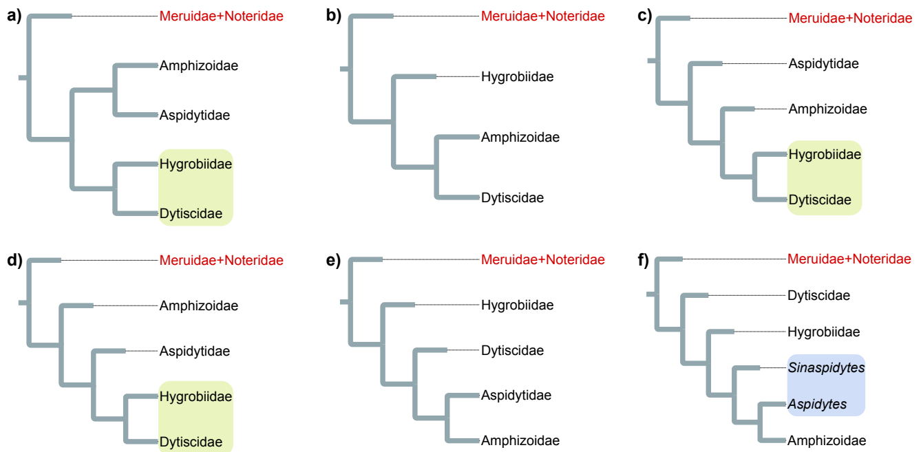
Fig. 1. Overview of different phylogenetic hypotheses on family phylogenetic relationships among Dytiscoidea proposed in previous studies that had analyzed molecular and morphological data. (Note that Meruidae were not included in all studies. However, since their sister group relationship to Noteridae is generally considered undisputed, we consistently included them in the overview: “Meruidae + Noteridae”). (a) Balke et al. (2005) based on morphological data, (b) Baca et al. (2017) based on UCE data, (c) Beutel et al. (2006, 2013) based on morphological data, (d) Ribera et al. (2002a) based on morphological and molecular data, (e) Balke et al. (2005, 2008) based on molecular data and Balke et al. (2005) based on morphological and molecular data, (f) Toussaint et al. (2015) based on molecular data and McKenna et al. (2015) based on molecular data with only Aspidytes included.
