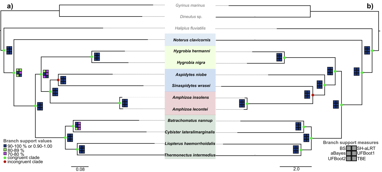
Fig. 3. Comparison of phylogenetic hypotheses resulted from the analysis of the codon-based nucleotide sequence data. Congruent and incongruent clades between the two trees (in terms of included terminal taxa) are illustrated in different colors. (a) Phylogram with the best log-likelihood score on the optimized scheme of supermatrix nt.A.homogeneous2. (b) Phylogram with the best log-likelihood score on the unoptimized partitioning scheme of supermatrix nt.A. Branch support is denoted based on 100 non-parametric bootstrap replicates (BS), 10,000 SH-like aLRT replicates (SH-aLRT), aBayes support, 1,000 Ultrafast Bootstraps 1 (UFBoot1), 1,000 Ultrafast Bootstraps 2 (UFBoot2, -bnni), and 100 bootstraps by transfer (TBE). Both trees were rooted with Gyrimidae.
