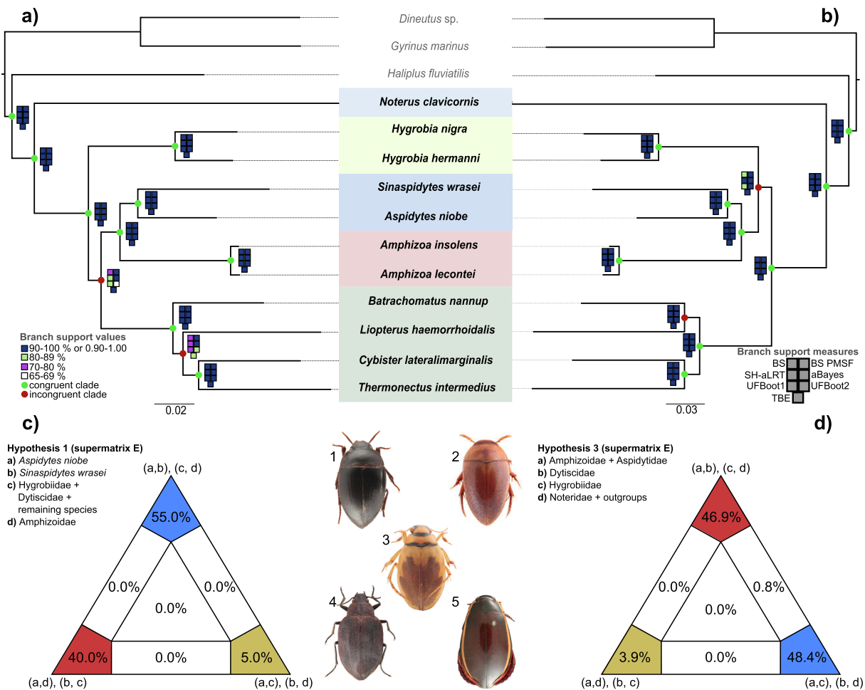
Fig. 2. Different phylogenetic hypotheses deduced from the analysis of amino-acid sequence data. (a) Phylogram with the best log-likelihood score on the optimized scheme of supermatrix H and (b) phylogram with the best log-likelihood score on the optimized scheme of supermatrix E. Branch support is denoted based on 100 non-parametric bootstrap replicates (BS), 100 non-parametric bootstraps based on the PMSF model (BS PMSF), 10,000 SH-like aLRT replicates (SH-aLRT), aBayes support, 1,000 Ultrafast Bootstraps 1 (UFBoot1), 1,000 Ultrafast Bootstraps 2 (UFBoot2, -bnni), and 100 bootstraps by transfer (TBE). Both trees were rooted with Gyrinidae. Congruent and incongruent clades between the two trees (in terms of included terminal taxa) are illustrated in different colors. (c) Results of the FcLM analysis on the original data of supermatrix E for the phylogenetic hypothesis 1 (i.e. monophyly of Aspidytidae). (d) Results of the FcLM analysis on the original data of supermatrix E for the phylogenetic hypothesis 3 (i.e. Hygrobiidae are the sister group of Amphizoidea + Aspidytidae). Beetle photos: (1) Sinaspidytes wrasei , (2) Noterus crassicornis , (3) Hygrobia hermanni , (4) Amphizoa lecontei , (5) Cybister lateralmarginalis (photos and copyright: M. Balke).
