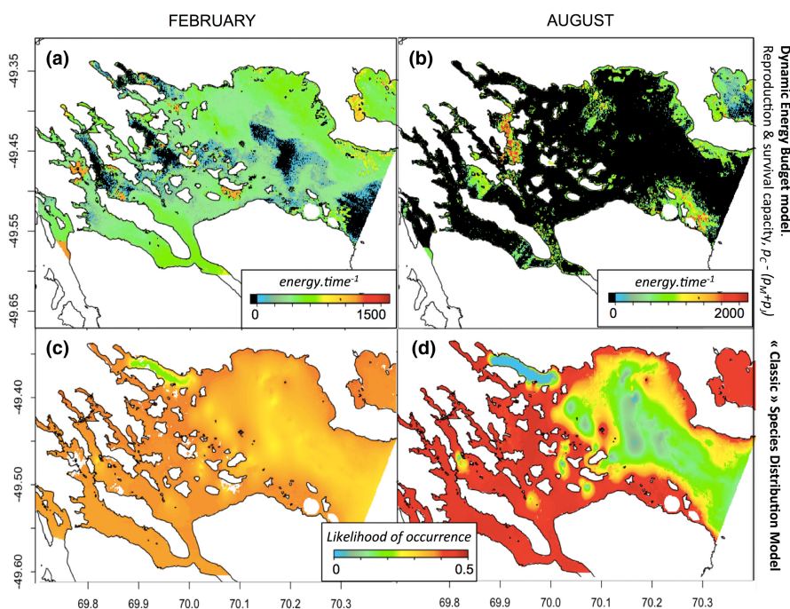
FIGURE 3 Spatial projections of the DEB model in February (a) and August (b). Reproduction and survival capacity is represented by the calculation of pC - (pM + pJ) (energy.Time -1 ), colour scale is given in energy.Time -1 , which indicates the possibility for reproduction and survival for values >0; or no possibility for reproduction and survival for values <0 (black). Spatial projections of the 'classic SDM' for February (c) and August (d), an average of 50 model replicates representing the average relative likelihood of occurrence. Relative likelihood values (possibly contained between 0 and 1) were capped at 0.5 for increasing figure readability.
