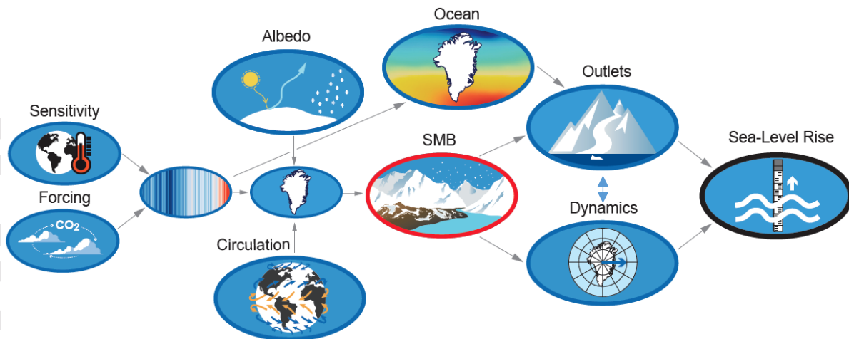
Fig 2: Causal relation between processes leading to a high-end contribution of Greenland to SLR. Critical processes are albedo, ocean forcing and atmospheric circulation changes. These three processes impact the SMB. Outlet glaciers change by changes in SMB and ocean forcing and SMB also influences the dynamics of the main ice sheet, where the ocean affects the outlet glaciers, together controlling the SLR.
