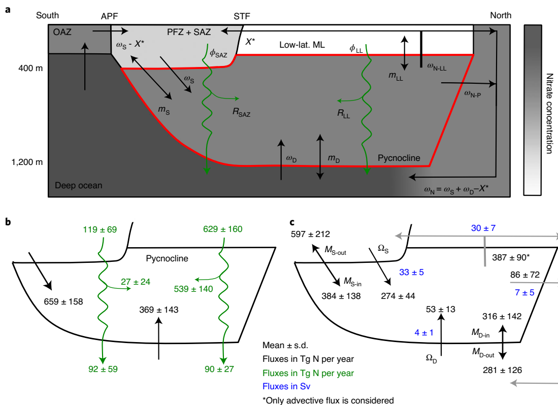
Fig. 1 | One-box model of the pycnocline for estimating water and nutrient transports and the model's results. Based on observations, the model solves for the steady-state conditions in the pycnocline. a , Schematic of the meridional overturning circulation showing the reservoirs and processes (Methods). Straight arrows represent water exchange terms, while curved arrows show export production and remineralization. b , Nitrogen fluxes, including the gross inputs of nitrate to the pycnocline (that is, \Omega + M_{in} , in Tg N per year) and export production and remineralization fluxes (in Tg N per year) (mean \pm s.d.). c , Deconvolution of advective and mixing components, \Omega and M (mean \pm s.d.), derived from the model best fits and prior estimates of the advective flows 38,39 ( \omega , in Sv and shown in blue). OAZ, Open Antarctic Zone; Low-lat. ML, low-latitude mixed layer.
