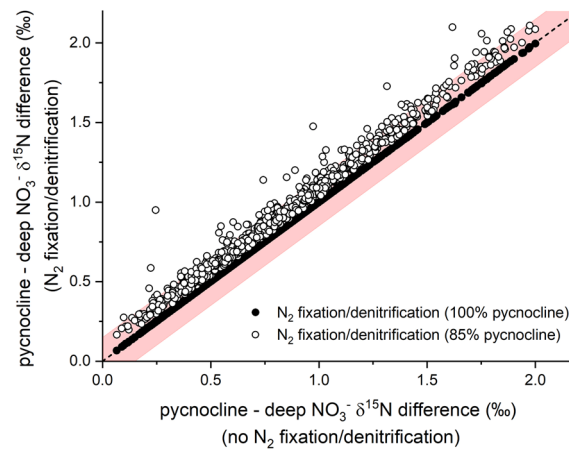
Extended Data Fig. 2 | Comparison of fixed N budget scenarios in the prognostic five-box ocean model. Comparison of the \text{NO}_3^- \delta^{15}\text{N} difference between the deep ocean and the pycnocline for the model scenario without \text{N}_2 fixation - denitrification and either the scenario where 20% of sedimentary denitrification (15% of total denitrification) occurs in the deep ocean, accompanied by a balancing amount of \text{N}_2 fixation (empty circles). The red envelope represents the uncertainty for the model best-fits given by the one-box model (Extended Data Figure 6c).
