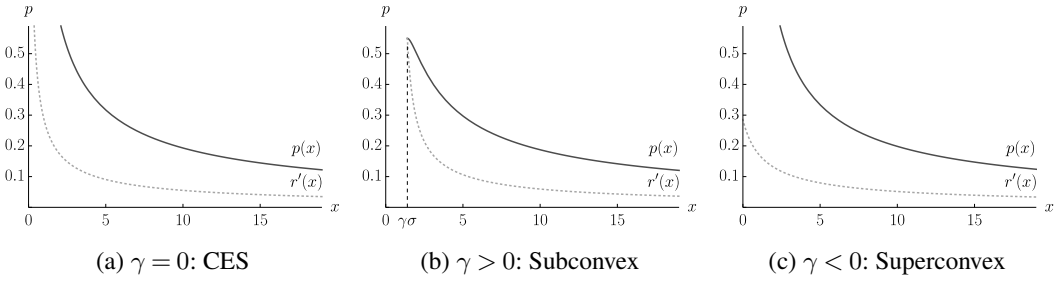
FIGURE 1.—Examples of CREMR demand and marginal revenue functions. Panels (a), (b), and (c) depict the CREMR demand from (6) and marginal revenue from (29) for \beta = 1 , \sigma = 1.4 , and for \gamma equal to 0, 1 and -1 respectively.
