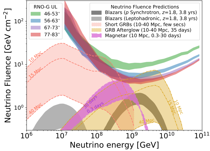
Figure 28. 95% CL fluence sensitivities between triggers at 1.5\sigma_{\text{noise}} and 2.5\sigma_{\text{noise}} are shown for four zenith bands centered at (top to bottom) 50^\circ (green), 60^\circ (blue), 70^\circ (purple), and 80^\circ (red). Sensitivities are calculated for a full decade in energy. Model-predicted fluences from several transient classes (bright gamma-ray blazars [132], short GRBs [130], magnetars [131], and GRB afterglows [49]) are also shown for direct comparison. We scale the short GRB and GRB afterglows by several luminosity distances to demonstrate the distance over which RNO-G will be sensitive to transients; a similar scaling can be applied to other source classes. For the calculation of sensitivities here we have used an integrated background expectation of no events. Note that for longer duration transients, integrated background may become non-negligible.
