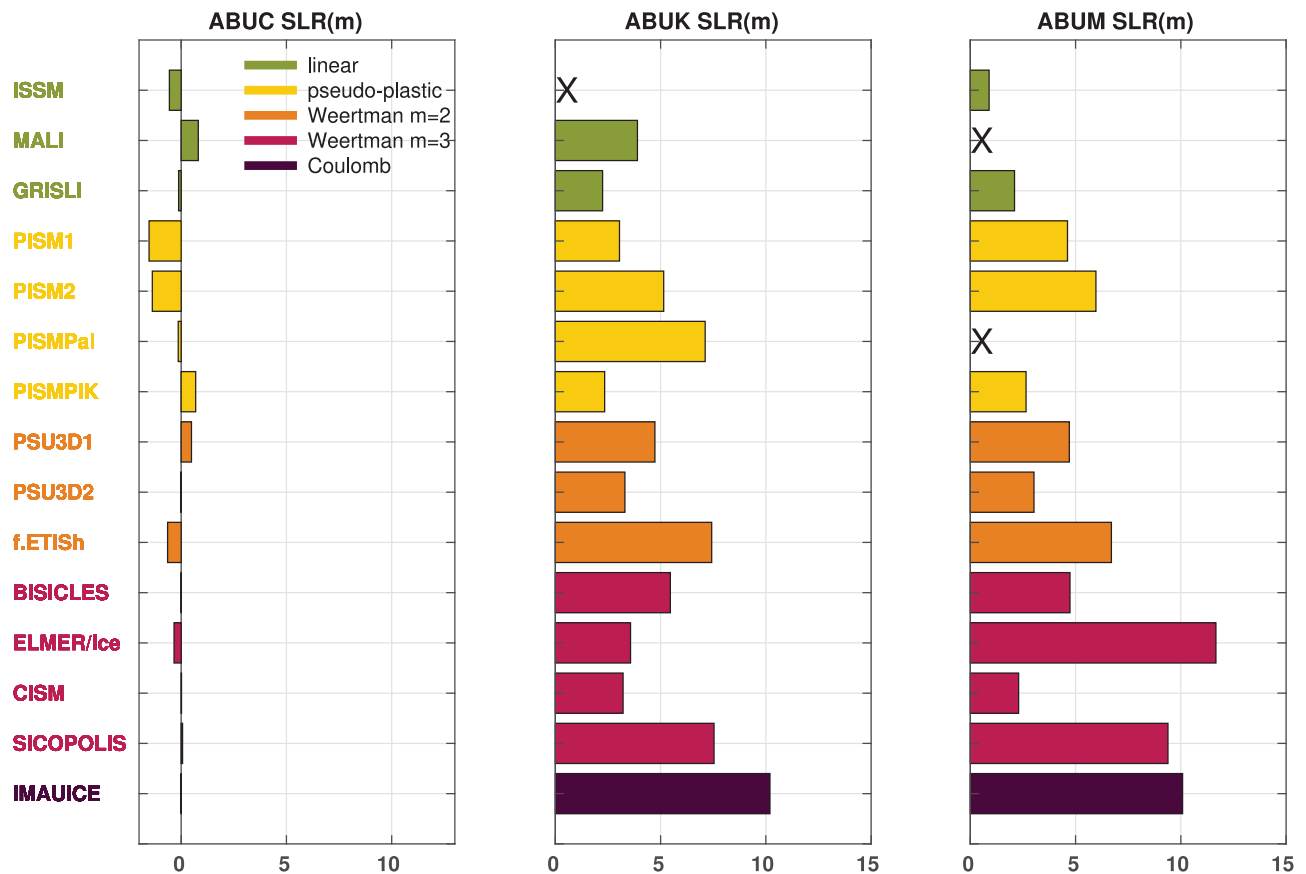
Fig. 5. Overall mass loss (volume above flotation; VAF) for the participating models ordered according to basal friction law characteristics: Weertman and Coulomb linear ( m=1, q=1 ), pseudo-plastic Coulomb ( q=0.6-0.75 ), Weertman m=2 , Weertman m=3 , Coulomb plastic q=0 . Models that did not participate a particular experiment are marked by 'X'.
