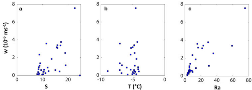
Fig. 12. Upwards brine velocities ( w ) vs. (a) bulk ice salinity ( S ), (b) bulk ice temperature ( T ) and (c) bulk ice Rayleigh number ( Ra ) for all 27 PIPERS stations. Each data point is a mean vertical value for the considered variables for a given ice core, at a given location.
