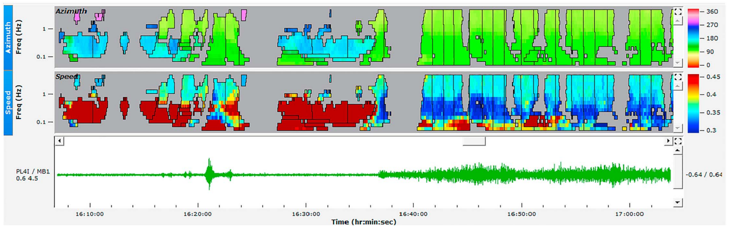
Figure 10. The upper and middle panels are time (x axis)-frequency (y axis) plots, with the colors corresponding to the azimuths (upper panel in degrees) and the speed (middle panel in m/s). Progressive Multi Channel Correlation (PMCC, Cansi, 1995; 15 log-spaced bands adapted from Matoza et al., 2013, and window lengths varying in proportion to the period from 30 to 250 s) results from the infrasound array installed in Pelabuhan Ratu (West Java) highlighting two clear signals starting at ~16:21 and 16:36 with an azimuth of ~90° pointing toward the Kelud volcano (upper panel) and typical acoustic speeds (~360 m/s, middle panel). The first signal is of short duration (a few minutes), while the second phase lasts for 2 hr (filtered between 0.1 and 5 Hz, lower panel).
