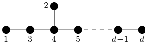
Figure 1. Dynkin diagram of E_d .
