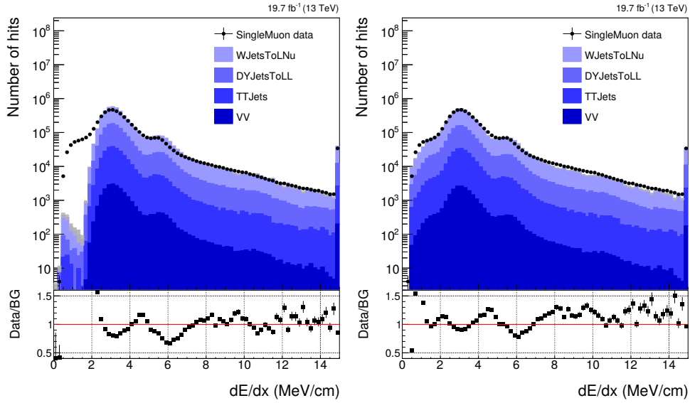
Figure D.4: dE/dx spectrum before (left) and after (right) corrections in the TEC in early 2016 data ( 19.7 \text{ fb}^{-1} ).
