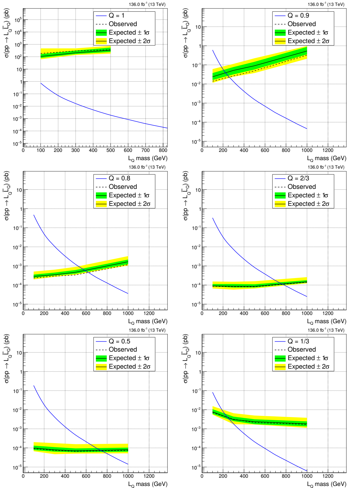
Figure 6.35: Limit on the Q = 1, 0.9, 0.8, 2/3, 0.5 and 1/3 signal cross-section using the full dataset. For Q = 1 , no limit is available for a signal of mass M = 1 \text{ TeV} as zero signal events are expected due to a lack of simulated events.
