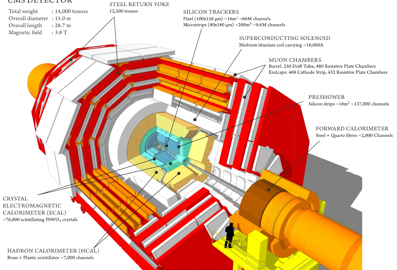
Figure 3.2: CMS and its subdetectors [71].
