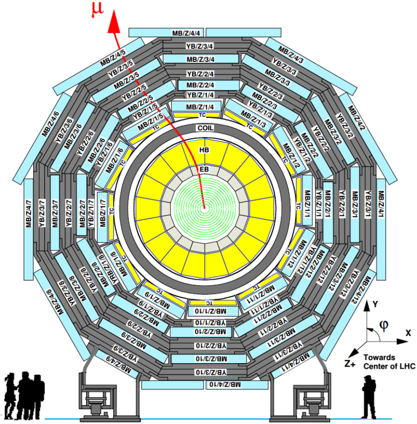
Figure 3.22: Geometry of the muon system (top) [80] and transverse view in the barrel (bottom) [70].
