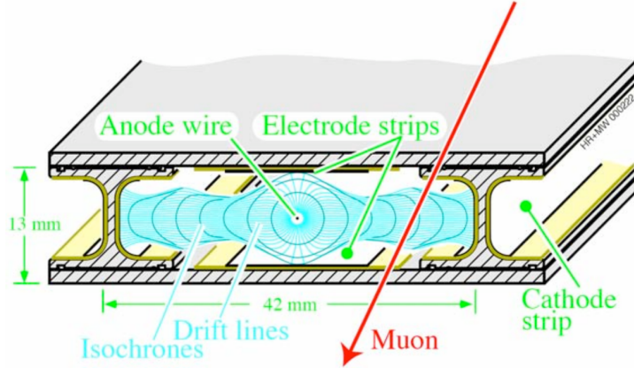
Figure 3.23: Illustration of a DT cell. [70].
