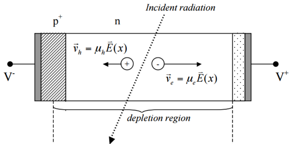
Figure 3.4: p-n junction (top) and typical configuration of a silicon-based sensor (bottom) [72]. On the right figure, V^\pm is the voltage, \vec{E} the corresponding electric field, \vec{v}_h is the drift velocity for the holes, \vec{v}_e is the drift velocity for the electrons and \mu_h and \mu_e are the corresponding mobilities.
