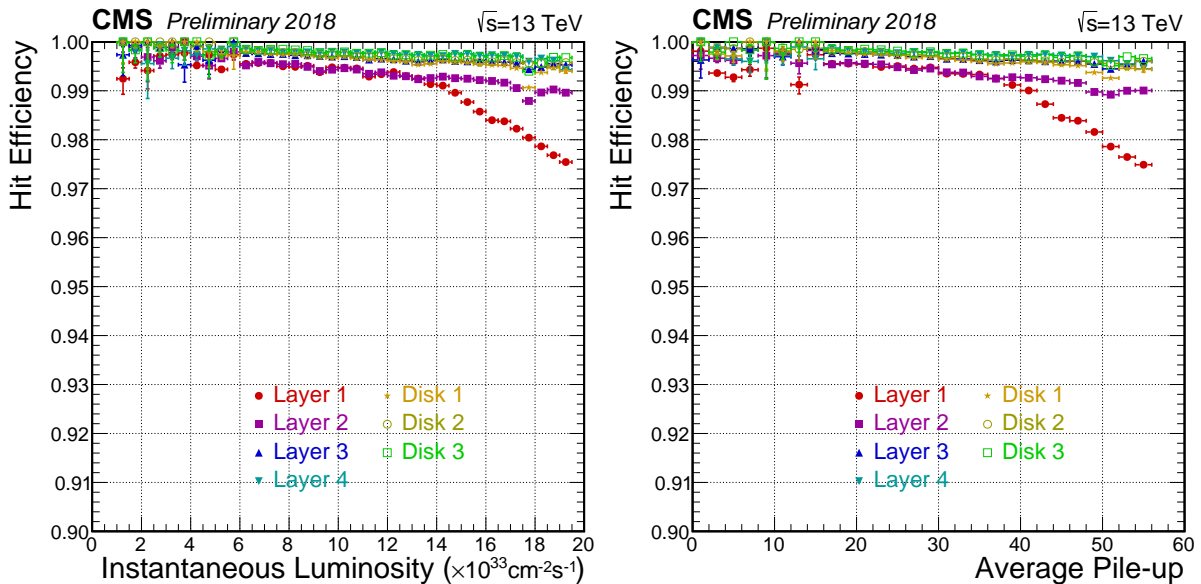
Figure 3.8: Average hit efficiency as a function of the instantaneous luminosity (left) and pileup (right) in 2018 data [74].
