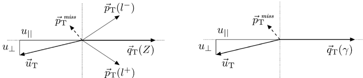
Figure 4.1: Z(\ell\ell) + jets (left) and \gamma + jets (right) events where \vec{q}_T is the boson transverse momentum and \vec{u}_T is the hadronic recoil, i.e. the transverse momentum of the jet system in the event [102]. The recoil is decomposed in the u_{\parallel} and u_{\perp} components respectively parallel and perpendicular to the boson \vec{q}_T .
