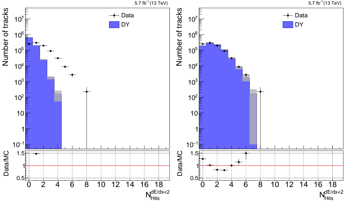
Figure 6.26: N_{\text{hits}}^{\text{dE}/\text{dx} < 2} in a subset of 2016 data compared with DY simulations before (left) and after (right) application of the corrections derived in section 6.8.3. We insist on the fact that the spectrum is not shifted by a global factor but that the changes are a propagation of the corrections applied on the \text{dE}/\text{dx} spectra for each layer.
