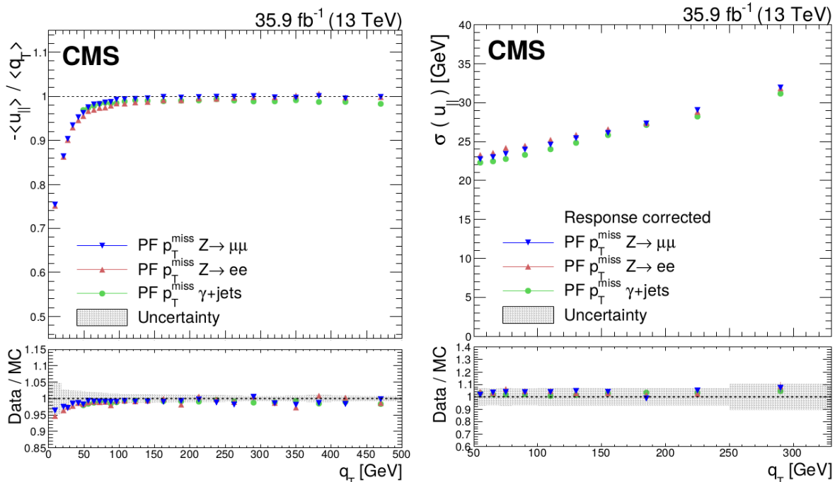
Figure 4.2: E_T^{\text{miss}} response (left) and resolution on the parallel component of the boson vector (right) for Z(\ell\ell) and \gamma + jets events in the full 2016 dataset [102].
