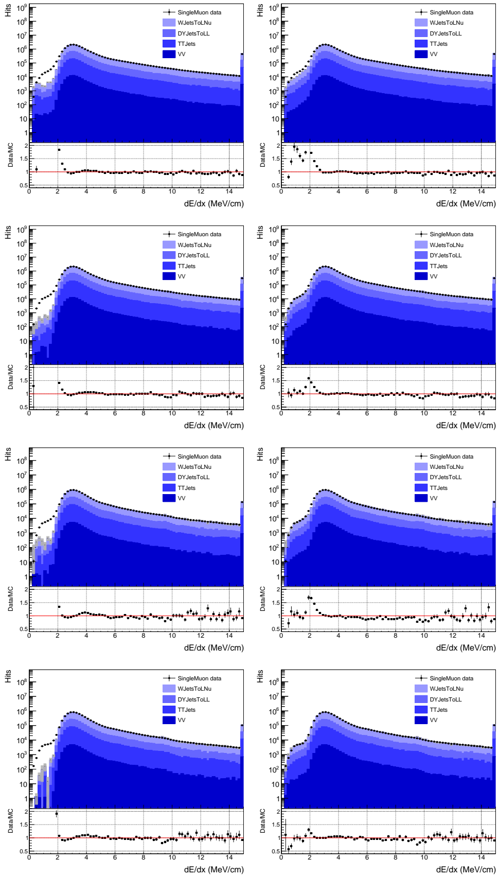
Figure D.14: dE/dx spectrum before (left) and after (right) corrections in the TIB layer 1 (top) to 4 (bottom) in 2018 data ( 58.8 \text{ fb}^{-1} ).
