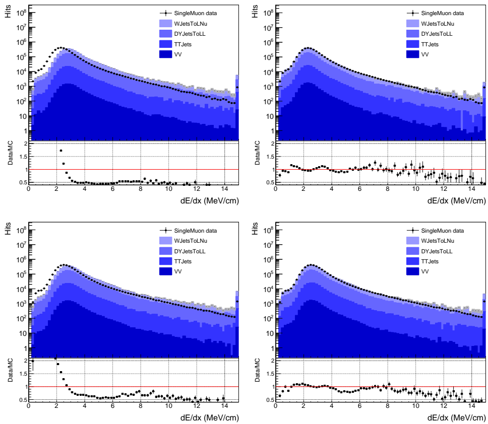
Figure D.5: dE/dx spectrum before (left) and after (right) corrections in the PXB layer 2 (top) and layer 3 (bottom) in late 2016 data ( 16.2 \text{ fb}^{-1} ).
