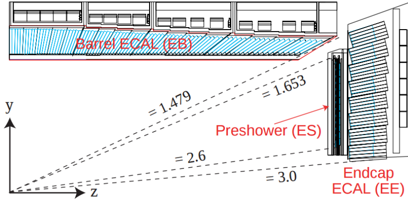
Figure 3.16: ECAL geometry [80].
