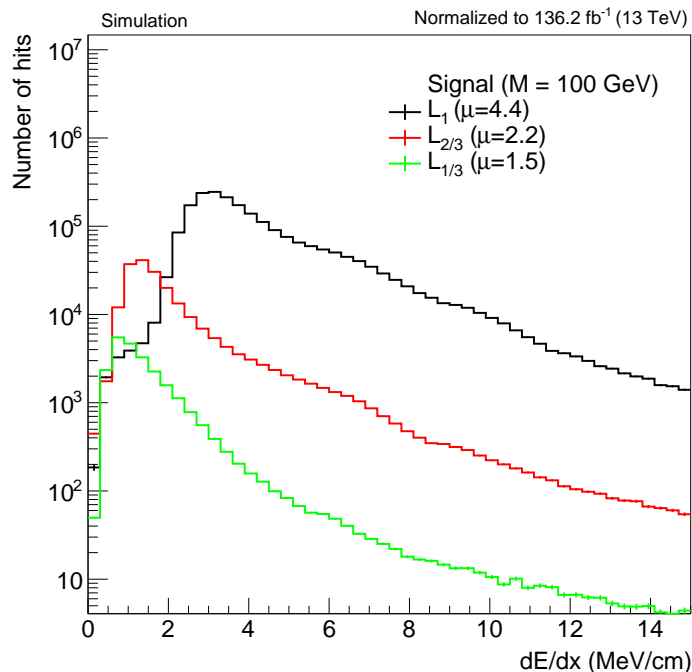
Figure 6.8: Stopping power spectrum for FCP of mass 100 GeV. The lower the charge, the lower the peak of the spectrum. The mean \mu of the distribution is also given.
