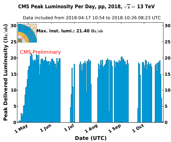
Figure 2.9: Peak instantaneous luminosity delivered per day by the LHC to CMS (left) and integrated luminosity delivered by the LHC and recorded by CMS per day (right) in 2016 (top), 2017 (middle) and 2018 (bottom) [64].
