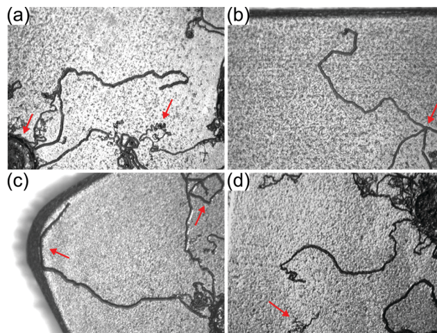
Fig. 1 Filiform corrosion patterns formed on coated low carbon steel under high relative humidity. Temperature: 38 °C. Field of view in all frames: 15.8 \times 11.8 \text{ mm}^2 . The red arrows highlight zones of interest described in the text.
