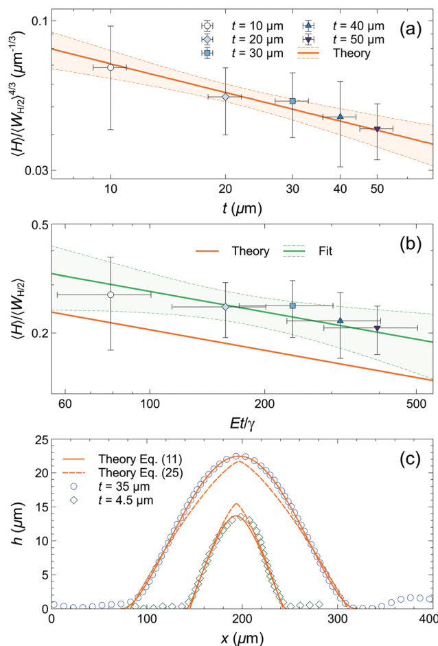
Fig. 6 (a) Evolution of \langle H \rangle / \langle W_{H/2} \rangle^{4/3} as a function of the thickness t . The error in t represents 10% of its mean value and reflects the uncertainty (0.5 \mu\text{m} ) for each applied layer of 5 \mu\text{m} . The best power law fit \alpha t^{-1/3} with \alpha = 0.15 \pm 0.03 is also shown together with the 95% confidence band. (b) Evolution of \langle H \rangle / \langle W_{H/2} \rangle as a function of the rescaled thickness Et/\gamma . The error in Et/\gamma originates from the uncertainties in E , \gamma (see eqn (1)) and t . The best power law fit \beta (Et/\gamma)^{-1/4} with \beta = 0.9 \pm 0.3 is shown together with the 95% confidence band and the theoretical scaling (31). (c) Comparison between the theoretical and experimental height profiles obtained by using the average parameter values eqn (1). The solid curves are theoretical profiles obtained by solving eqn (11) with P = 4.7 \times 10^7 \text{ Pa} for t = 35 \mu\text{m} and P = 1.1 \times 10^7 \text{ Pa} for t = 4.5 \mu\text{m} . The dashed curves are theoretical profiles obtained in the asymptotic limit of large pressure using eqn (25) and (30) with P = 7.5 \times 10^6 \text{ Pa} for t = 35 \mu\text{m} and P = 1.05 \times 10^7 \text{ Pa} for t = 4.5 \mu\text{m} .
