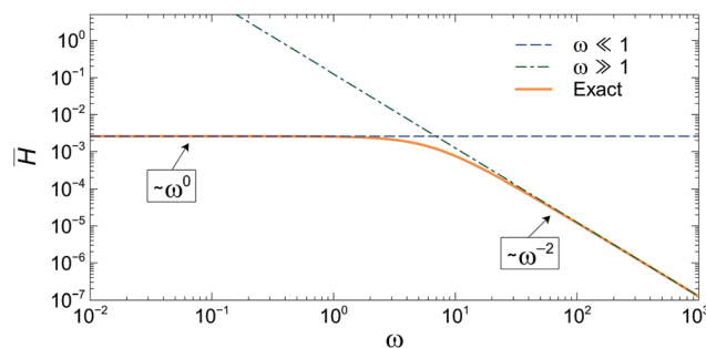
Fig. 4 Evolution of \bar{H} given by eqn (20) as a function of \omega given by eqn (17a). The asymptotic expressions (21b) are also shown.
