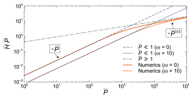
Fig. 5 Evolution of \bar{H}\bar{P} as a function of \bar{P} obtained by solving numerically eqn (16) for two values of \omega together with the asymptotic expressions (20) and (26).
