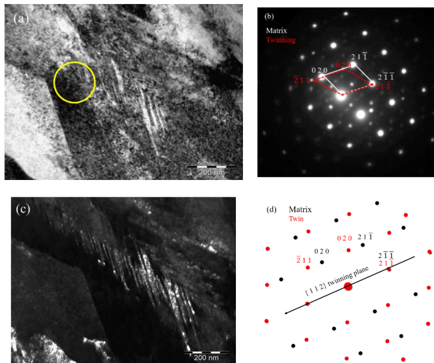
Figure 7. (a) A BF image of the WEL surface in the TEM foil; (b) Selected area diffraction (SAD) pattern, corresponding to zone axis [102]matrix of the region enclosed in the yellow circle; The (c) DF image formed from the (\bar{2}11) reflection of the twinning plane and (d) simulated diffraction pattern corresponding to (b).
