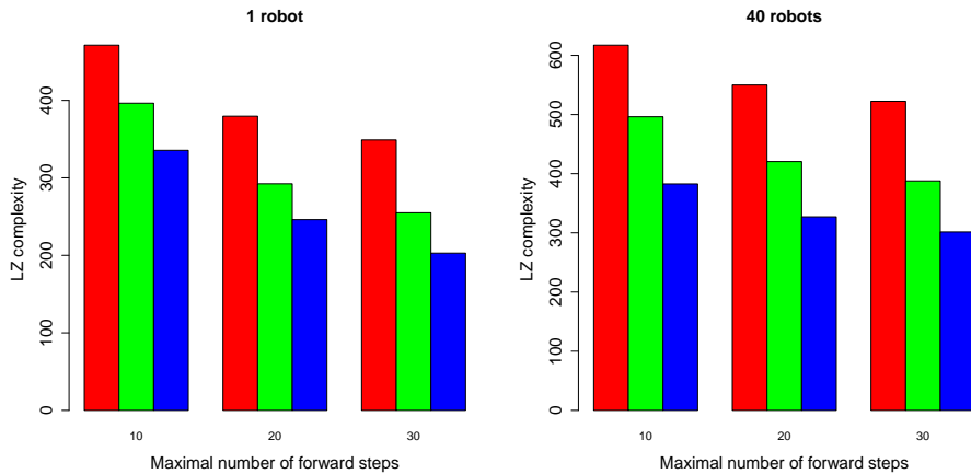
Fig. 2. LZ complexity for the case with 1 robot (left) and 40 robots (right) in the dodecagonal arena. Maximum turning angles: ■ 40^\circ ■ 90^\circ ■ 180^\circ
