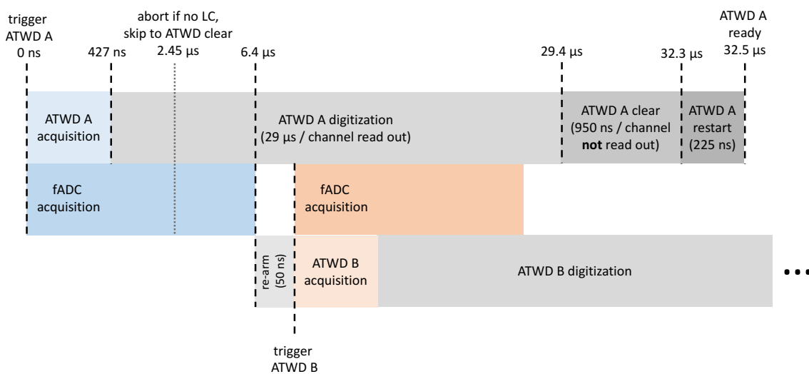
Figure 7. Timing of ATWD and fADC acquisition and associated deadtime, for back-to-back HLC hits with one ATWD gain channel of four digitized and read out. The horizontal (time) axis is not to scale.
