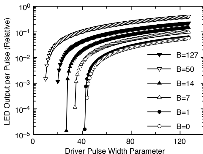
Figure 9. Light output from flasher LED pulses (relative to maximum), depending on brightness parameter (B) and width configuration parameters. Additional dynamic range is available by enabling from 1 to 12 individual LEDs per DOM.
