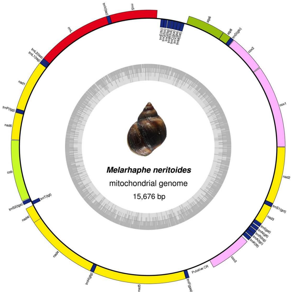
Fig 1. Gene map of the Melarhappe neritoides mitogenome. Genes encoded on the H strand are mapped outside the outer circle and are transcribed counterclockwise. Genes encoded on the L strand are mapped inside the outer circle and are transcribed clockwise. The inner circle plot represents G + C% content; the darker lines are, the higher their G + C% is. Photo credit: Yves Barette (RBINS).
