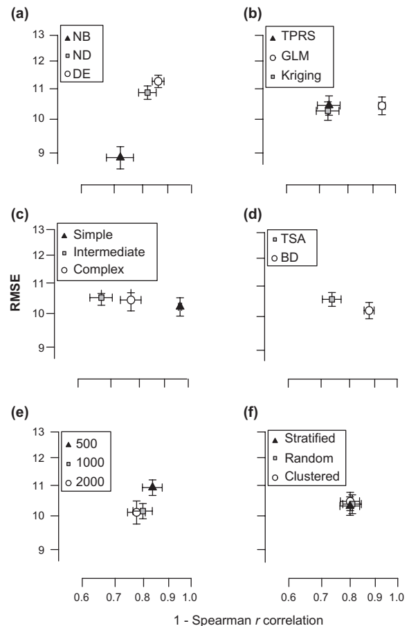
Figure 5. Relationships between averaged RMSE and Spearman correlation values with 95% confidence levels broken-down for the six tested factors: (a) spread rate estimator, (b) interpolation model, (c) pattern of invasion, (d) spatio-temporal modelling structure, (e) numbers of samples and, (f) the sample spatial distribution.
