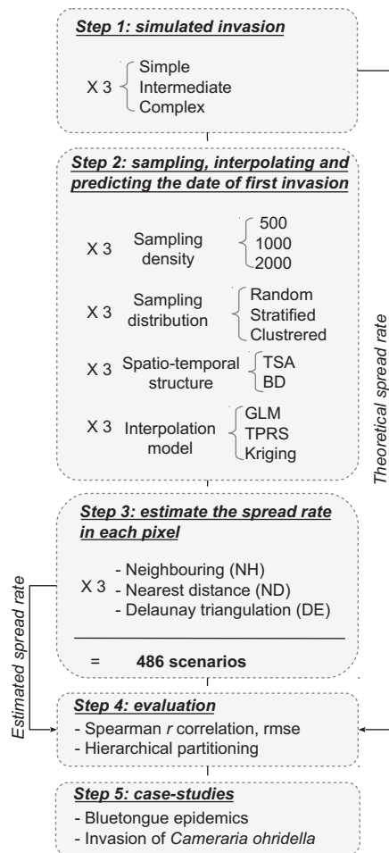
Figure 1. Summary of methods employed to evaluate different spread rate estimators.
