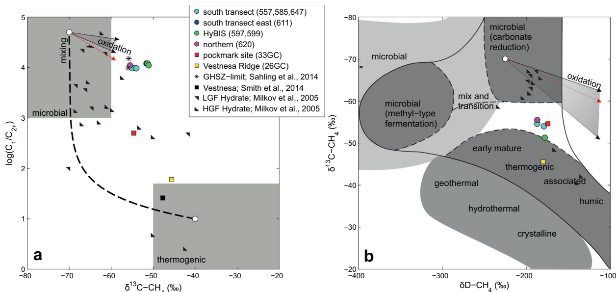
Fig. 6. Molecular and isotopic composition of hydrate and bubble plume gases from this study (coloured symbols) and others (black symbols). (a) ‘Bernard diagram’ modified after Whiticar (1999), (b) Cross plot of methane carbon and hydrogen isotopic data with classification according to Whiticar (1999). White open circles indicate typical end member microbial ( \delta^{13}\text{C}-\text{CH}_4 : -70 ‰, C_1/C_{2+} : 50,000, \delta\text{D}-\text{CH}_4 : -225 ‰, in A and B) and thermogenic (A only: \delta^{13}\text{C}-\text{CH}_4 : -40 ‰, C_1/C_{2+} : 10) source signatures, connected by a black dashed mixing line (A only). Shaded area between the black arrows shows the effect of oxidation on \delta^{13}\text{C}-\text{CH}_4 and \delta\text{D}-\text{CH}_4 for the range of isotope fractionation factors ( \alpha_C for carbon and \alpha_D for hydrogen) reported from laboratory experiments with aerobic and anaerobic methanotrophic bacteria (Feisthauer et al., 2011; \alpha_C : 1.012–1.036, \alpha_D : 1.093–1.320). Red arrows show \alpha_C and \alpha_D values measured in aerobic sediments from the northern Baltic Sea (Egger et al., 2015; \alpha_C : 1.009, \alpha_D : 1.098). Vestnesa Ridge hydrate \delta^{13}\text{C}-\text{CH}_4 data are from Fisher et al. (2011). Previously reported Vestnesa Ridge hydrate (Smith et al., 2014), and LLGHSZ bubble plume data (Sahling et al., 2014), as well as hydrate data from both high gas flow (HGF) and low gas flow (LGF) regions (Milkov et al., 2005), are also shown. (For interpretation of the references to colour in this figure legend, the reader is referred to the web version of this article.)
