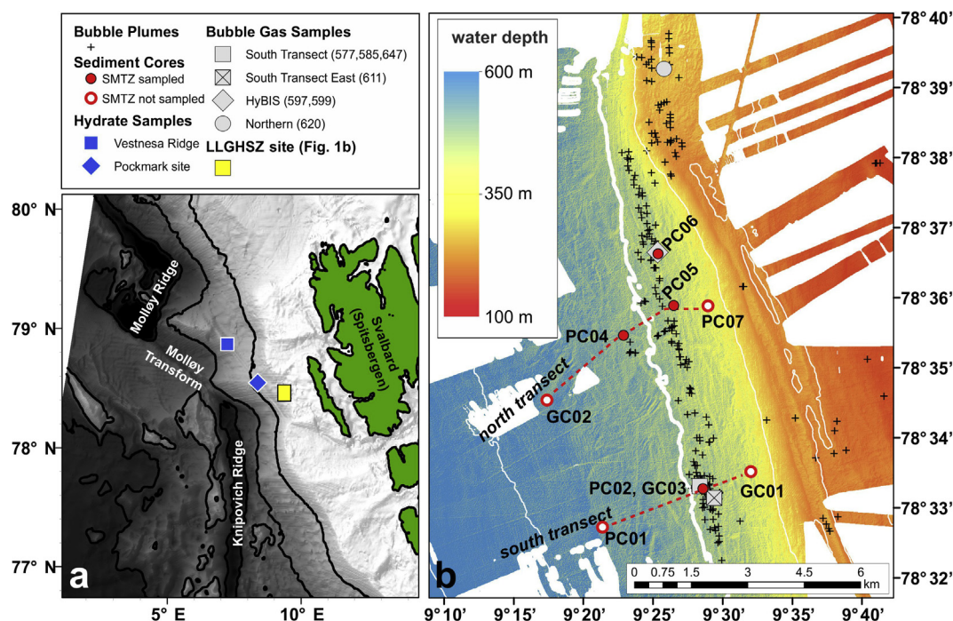
Fig. 1. Location of the West Svalbard continental margin and the study area. (a) Regional map indicating the locations of hydrate samples (blue symbols) and the main study site (LLGHSZ, yellow rectangle), bathymetry data from GEBCO (The GEBCO_08 Grid, version 20100927, http://www.gebco.net ) with 1,000 m depth contours. (b) Main study site at the LLGHSZ, showing shipboard bathymetry (cruise JR253), 100 m depth contours (white lines) with 400 m in bold, seafloor gas bubble plumes mapped during JR253 (black crosses), sediment core locations (red circles), and bubble plume sampling sites (grey symbols). (For interpretation of the references to colour in this figure legend, the reader is referred to the web version of this article.)
