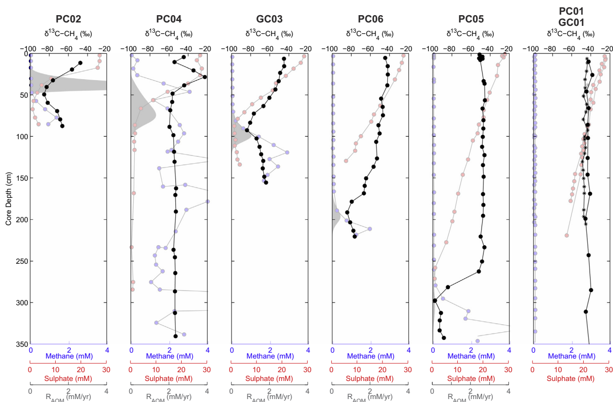
Fig. 3. Profiles of sediment methane carbon isotopic ratio ( \delta^{13}\text{C}\text{-CH}_4 ). Profiles of methane (blue) and sulphate (red) concentrations, and modelled rates of anaerobic oxidation of methane (grey shaded areas, see Section 4.3) are also shown. (For interpretation of the references to colour in this figure legend, the reader is referred to the web version of this article.)
