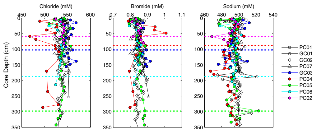
Fig. 4. Pore water profiles of chloride, bromide and sodium. Cores collected from less than \sim 0.01 to 0.3 km away from active bubble seeps are shown by the coloured symbols. Dashed horizontal lines indicate the depth of the SMTZ, where sampled.
