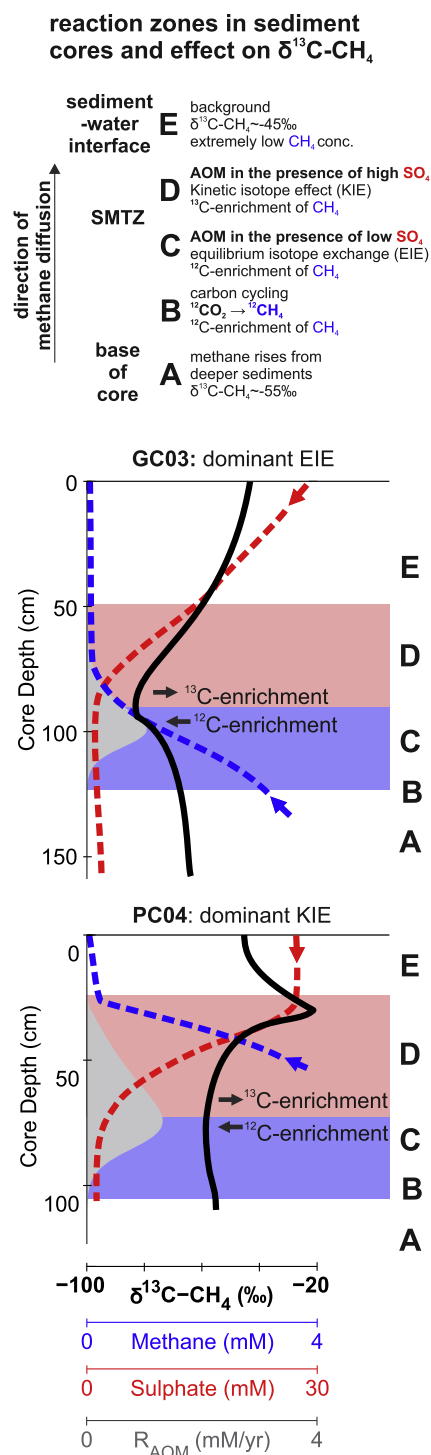
Fig. 7. Schematic illustration of the processes driving shifts in \delta^{13}\text{C}-\text{CH}_4 near the SMTZ. The interval in which AOM occurs (grey shaded area, modelled AOM rate as shown in Fig. 3), is divided into two zones: the upper area (pink, zone D) where AOM occurs in the presence of high sulphate concentrations favouring kinetic isotope fractionation, and the lower area in which AOM occurs in the presence of low sulphate concentrations favouring enzyme-mediated equilibrium isotope exchange (blue, zone C). (For interpretation of the references to colour in this figure legend, the reader is referred to the web version of this article.)
