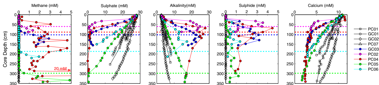
Fig. 2. Profiles of pore water methane, sulphate, alkalinity, sulphide and calcium. Cores collected from less than ~0.01 to 0.3 km away from bubble plumes are shown by the coloured symbols. Dashed horizontal lines indicate the depth of the SMTZ, where sampled. Sulphide was not determined in cores GC01 and PC07. (For interpretation of the references to colour in this figure legend, the reader is referred to the web version of this article.)
