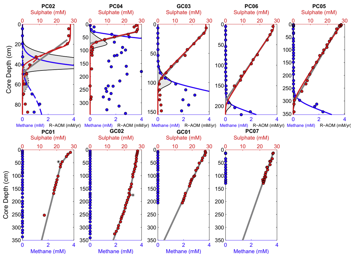
Fig. 5. Modelled pore water profiles: methane (blue), sulphate (red) and anaerobic methane oxidation rate ( R_{AOM} , grey shading). Measured data are shown by the coloured circles. Results of the diffusion-only model are shown by the solid grey lines (sulphate only, R^2 values given in Table 4). Results for the transport-reaction model for sulphate and methane are shown, respectively, by the red and blue lines. Black dashed lines for PC02 show the results of transport-reaction modelling with high advective flow (see Table 4). The maximum rate of AOM rate modelled in core PC02 is 9.9 \text{ mM yr}^{-1} ( 30 \text{ nmol cm}^{-3} \text{ day}^{-1} ). (For interpretation of the references to colour in this figure legend, the reader is referred to the web version of this article.)
