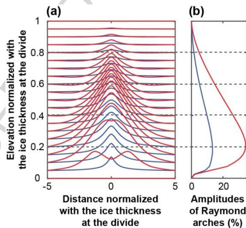
Figure 9 (one column): Properties of Raymond arches. (a) Cross section of modeled isochrones. (b) Depth variations of the arch amplitudes relative to the ice thickness at the divide. In both panels, blue shows a case of isotropic ice resulting in single-peak Raymond arches, and red shows a case of anisotropic ice induced by development of ice-crystal alignments resulting in double-peaked arches. The figure shows steady-state model results presented in Fig. 11b of Martin et al. (2009a).
