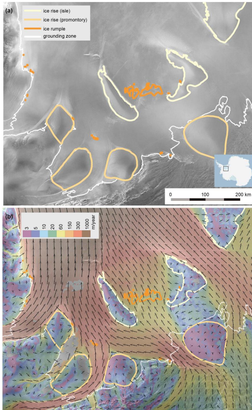
Figure 1 (2 columns): Ice rises and rumples in the Ronne-Filchner Ice Shelf, West Antarctica. Inset shows the location. Outlined are ice rises and rumples inventoried in this study (see Appendix). Bed topography in this region and names of these ice rises and rumples are shown in Figure 6b. The grounding zone of the ice sheet is also shown (Bindschadler et al., 2011). (a) Morphological structures associated with ice rises and rumples visible in Radarsat-2 satellite imagery (Jezek et al., 2002). Brightness changes are associated with surface-slope variations of major ice rises, as well as crevasses and rifts in the ice shelf. (b) Ice flow field (Rignot et al.,
