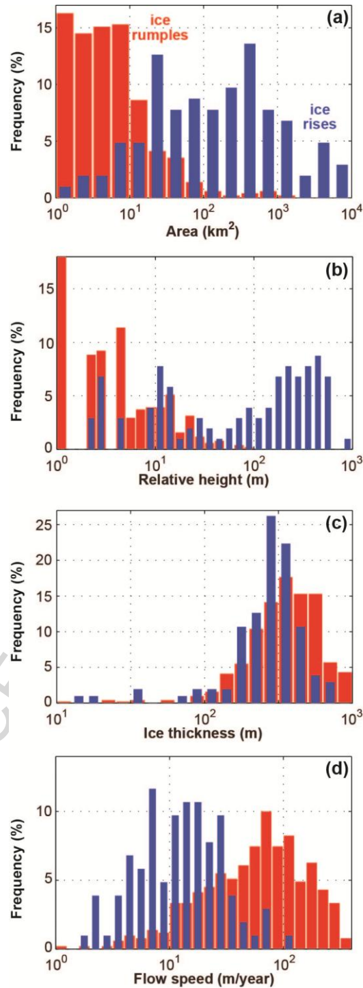
Figure 4 (one column): Population characteristics of ice rises and rumples. Panels show histograms of (a) area, (b) relative height of the highest place (summit) of ice rises/rumples measured from the adjacent ice shelf/stream surface, (c) maximum ice thickness, and (d) maximum flow speeds within the ice rises and rumples. All abscissas have a logarithm scale, and frequency is shown in percent of a total of the 103 isle-type ice rises and 510 ice rumples inventoried in this study (Table 1).
