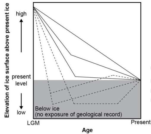
Figure 8 (one column): Surface-elevation changes of the ice sheet upstream of ice rises, associated with the ice-rise formation mechanisms shown in Fig. 7. Solid lines show cases of long-term stable and deglacial emergent (Figs. 7a and 7b). Dashed lines show GIA and glaciological emergent (Figs. 7c and 7d). Elevation changes in the shaded area occur below the current ice surface so geological records are not exposed.
