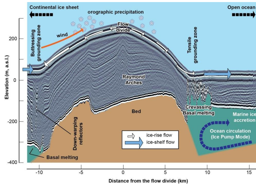
Figure 2 (2 columns): Cross section of an ice rise. The radargram is from an along-flow, ground-based profile across the summit of Kupol Ciolkovskogo near the Fimbul Ice Shelf, Dronning Maud Land (K. Matsuoka and J. Brown, unpublished data). Dominant wind direction is oblique to the cross section, and seabed beneath the ocean cannot be detected using radar. The sketches of orographic precipitation and seabed are included for illustration purposes.
