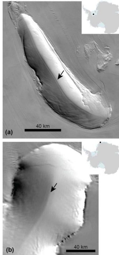
Figure 5 (one column): Near-parallel lineations (shown with arrows) along the ice-flow divide detected by MODIS satellite imagery (Haran et al., 2005; Scambos et al., 2007). Other lineations in the flank are often associated with the slope changes. (a) Korff Ice Rise in the Weddell Sea (Smith, 1986), which has a (single-peaked) Raymond arches (J. Kingslake, unpublished data). (b) Halvfarryggen Ridge in Dronning Maud Land, which has double-peaked Raymond arches (Drews et al., 2013). For Raymond arches, see Section 4.1.
