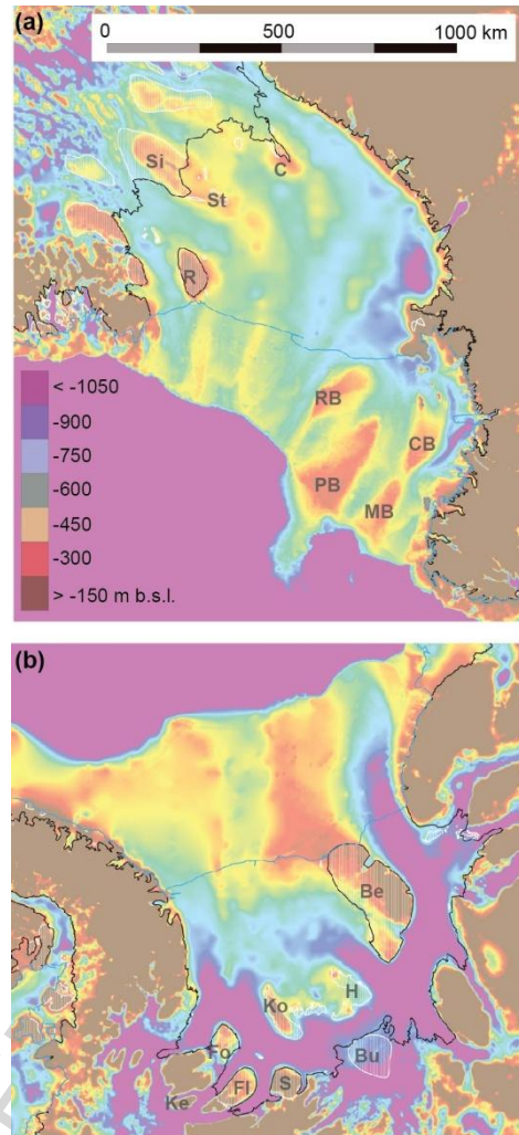
Figure 6 (one column): Elevated bed topography beneath ice rises and rumples in the Ross (a) and Weddell (b) Sea Embayments. Bed elevations are referenced to the GL04C geoid (Fretwell et al., 2013); geoid heights are ~40 m in the Ross Sea and ~20 m in the Weddell Sea. Outlined are the grounding zone (black; Bindschadler et al., 2011) and current ice-shelf's calving front (blue; Scientific Committee on Antarctic Research, 2012). Inventoried ice rises and rumples (Appendix) are hatched, and labels are given to major ice rises. In Panel (a), labeled are Siple Dome (Si), Roosevelt Island (R), Crary Ice Rise (C), and Steershead Ice Rise (St), as well as likely locations of ice rises during the LGM (Shipp et al., 1999): Crary Bank (CB), Mawson Bank (MB), Pennell Bank (PB) and Ross Bank (RB). In panel (b), labeled are the current ice rises and rumples: Berkner Island (Be), Henry Ice Rise (H), Korff Ice Rise (K), Bungenstock Ice Rise (Bu), Skytrain Ice Rise (S), Kealey Ice Rise (Ke), Fletcher Promontory (Fl), and Fowler Peninsula (Fo).
