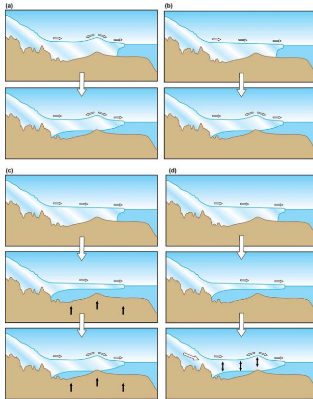
Figure 7 (1.5 column): Possible formation mechanisms for isle-type ice rises. (a) Long-term stable. (b) Deglacial emergent. (c) GIA emergent. (d) Glaciological emergent. For each case, the evolution is shown in scenes connected by large open downward arrows between panels. Open arrows within individual panels illustrate the direction of ice flow, whereas solid black arrows illustrate the emerging bed associated with GIA (c) and a thickening ice shelf (d). Corresponding changes of ice elevation are shown in Fig. 8.
