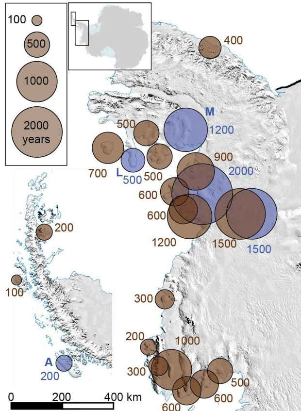
Figure 10 (one column): Twenty three ice rises in the Antarctic Peninsula and Amundsen Sea coast that show a pair of distinct near-parallel lineations in satellite imagery in the central part of the ice rise (similar to those shown in Fig. 5). Inset shows the location. Numbers are the characteristic ice-flow time scale T (= H/b in years, where H is ice thickness and b is SMB). The five ice rises shown with blue circles have well-developed, double-peaked Raymond arches (Fig. 9a); Adelaide Island (labeled as A), Latady Island (L) and Monteverdi Peninsula (M) were surveyed with ground-based radar and the other two with airborne radar. Background satellite image is Landsat (Bindschadler et al., 2008), and the calving front is highlighted in blue (Scientific Committee on Antarctic Research, 2012).
