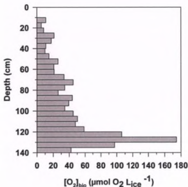
Figure 7 [O_2]_{bio} in BRW10 calculated following equation 3. The results may be converted into C uptake, assuming a photosynthetic quotient O_2/C of 1.43 [Glud et al. , 2002].
