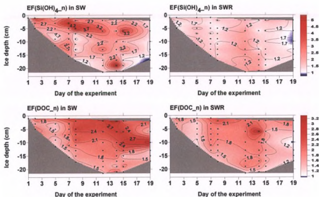
Figure 5. Evolution of the enrichment factor (EF) of \text{Si(OH)}_4_n and \text{DOC}_n in ice, between SWR and SW mesocosms. The black dots are depth-interpolated data points, while the colors in between are interpolations (natural neighbor).
