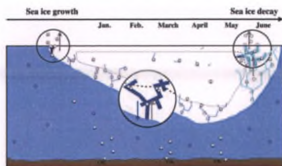
Figure 4. Schematic figure of \text{CH}_4 incorporation and release in sea ice. Sizes are intentionally disproportionate to highlight processes better. The area above the dotted line represents the impermeable layers. The small filled and empty circles represent \text{CH}_4 in gas bubbles and in dissolved state respectively. Upward grey arrows indicate the upward transport of gas bubbles due to their buoyancy, while downward blue arrows indicate the removal of dissolved gas through brine drainage. Large black circles zoom in on particular processes described in the text (Sect. 4.2): gas exchanges at the beginning of ice growth, gas accumulation predominantly under the impermeable layers and gas bubble escape during ice decay. Dark blue, light blue and cyan strokes in ice represent brine channels with high, moderate or low salinity respectively.
