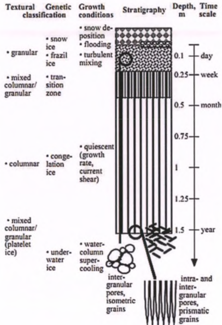
Figure 2 Scheme summarizing the main ice textures encountered in different ice growth conditions and at time scales for first-year ice [Petrich and Eicken, 2010]
