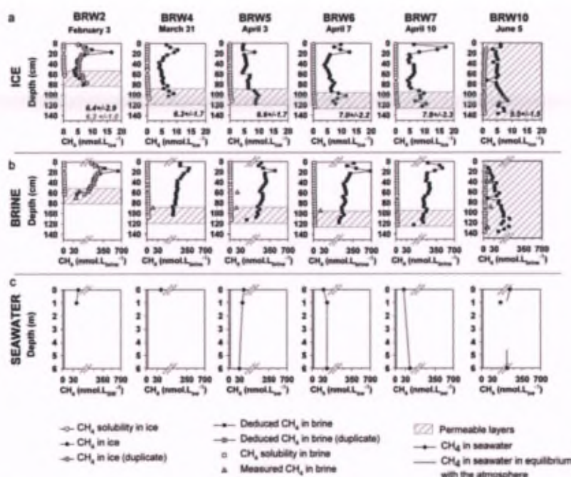
Figure 3. Evolution of \text{CH}_4 concentration in (a) bulk ice, (b) brine and (c) seawater (black dots, squares and diamonds respectively), compared to \text{CH}_4 solubility in ice, brine and seawater that is in equilibrium with the atmosphere (white dots, white squares and black straight lines respectively). Grey dots and grey squares are measurements made on duplicate samples of BRW2. Grey triangles in (b) are \text{CH}_4 measurements in brine sackholes. The break in the x axes of (b) and (c) is set at 60 nmol \text{L}^{-1} . Dashed areas are permeable layers (i.e. layers with a brine volume fraction above 5%).
