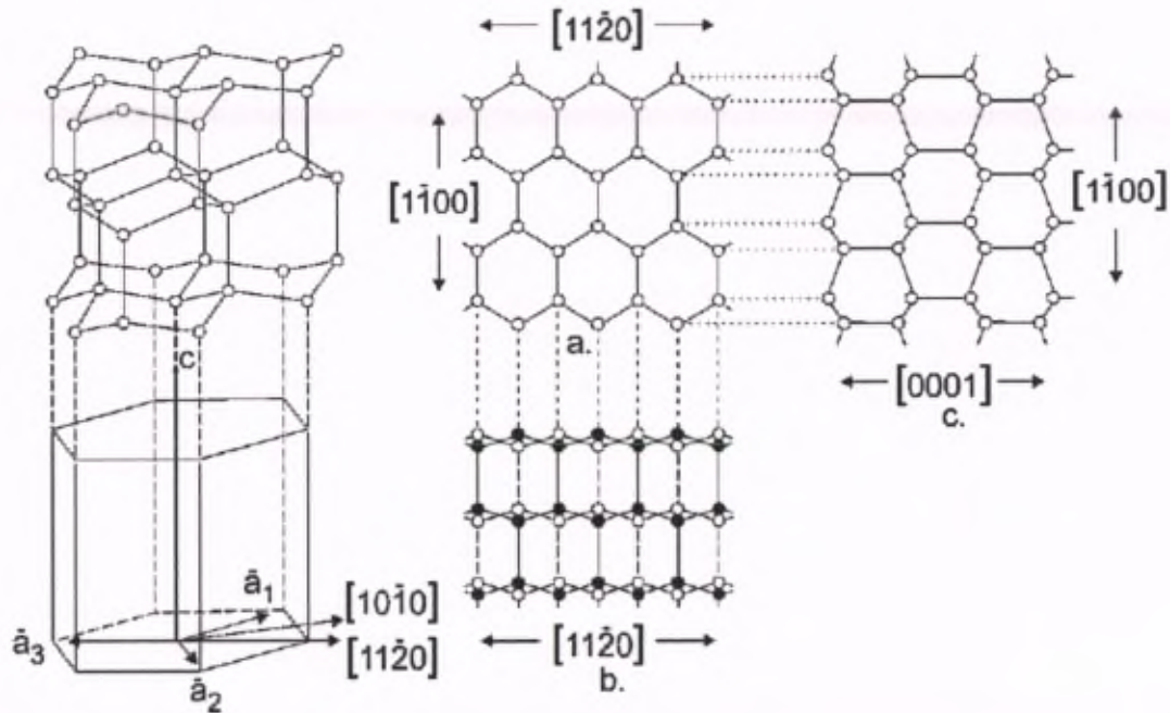
Figure 1 Crystal structure of sea ice (from Weeks and Ackley [1986]) on the left. The central panel presents the arrangement of oxygen atoms along (top) and perpendicular (bottom) to the c -axis (symmetry axis of order-6). The 3 a -axes (symmetry of order-2) are lying within the basal plane (left panel).
