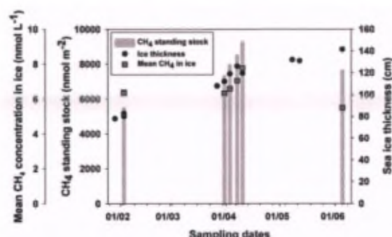
Figure 2. \text{CH}_4 standing stock for selected samplings events (vertical bars, from left to right, BRW2, BRW4, BRW5, BRW6, BRW7 and BRW10) in parallel with mean \text{CH}_4 concentration in sea ice and sea ice thickness.
