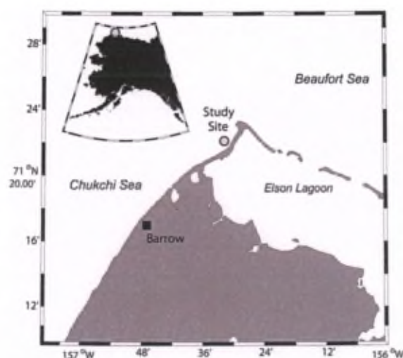
Figure 1. The study site, North of Barrow, Alaska, USA.
