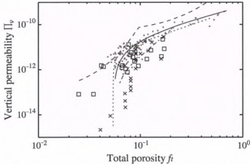
Figure 8 Vertical permeability as a function of total porosity from Petrich et al. [2006]. Relationships are from Petrich et al. [2006] (solid), Eicken et al. [2004] (dashed) and Freitag [1999] for young and old ice (dash-dot and dotted lines respectively). The data points are from Saeki et al. [1986] (squares), Maksym and Jeffries [2000] (crosses) based on Ono and Kasai [1985] and Saito and Ono [1978], and Cox and Weeks [1975] (grey dots).
