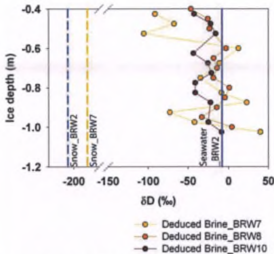
Figure 7. Calculated \delta D changes in brine below 40 cm depth at BRW7, BRW8, and BRW10 (see equation (4) in the text). \delta D in seawater, snow, and brines are plotted for comparison.
