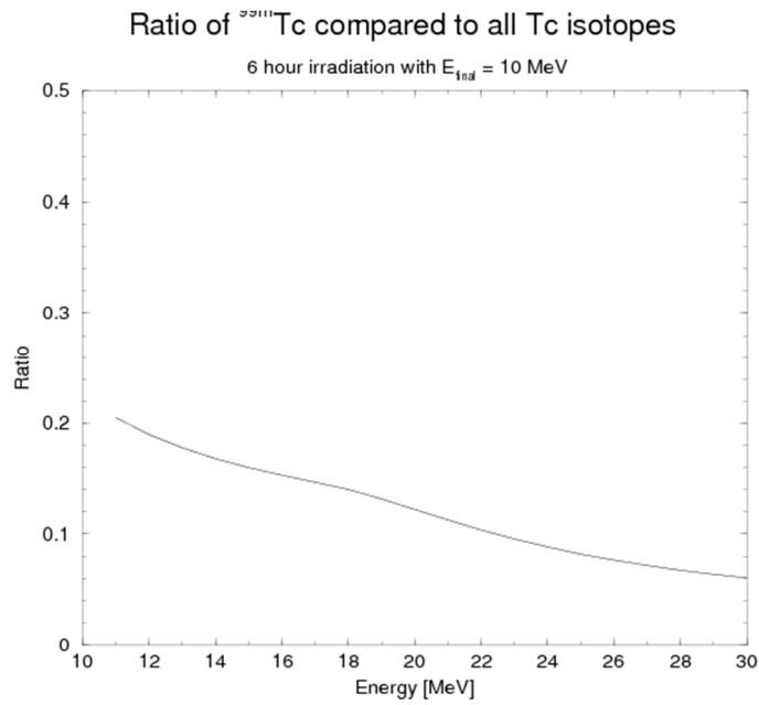
Figure 2: Radioactive yield and purity of Tc99m produced with protons on Mo100.
