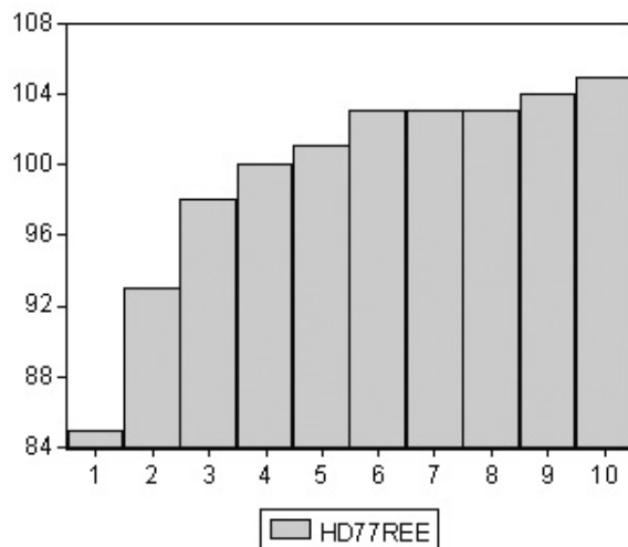
Figure 7: Empirical CDF of REE hitting lower limits
