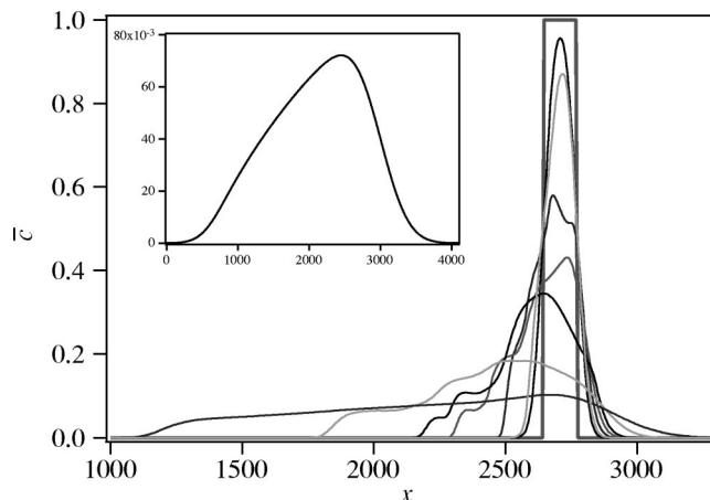
FIG. 3. Transverse average profiles of concentration at successive times t=0, 500, 700, 1000, 1500, 2000, 5000 , and 15000 . Inset: transverse average profile of concentration at t=60000 ( Pe=512, l=128, R=2, \varepsilon=1 ).
